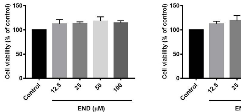
Figure 1. The cell viability of END and ENL on RAW264.7.
