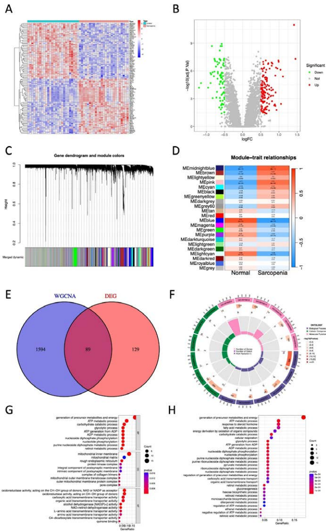
Figure 1. Genes differentially expressed between the sarcopenia and normal groups. (A) Heat map for differential expression analysis of GSE8479. (B) Volcanic map for differential expression analysis of GSE8479. Green represents downregulated genes, red represents upregulated genes, and black represents undifferentiated genes. (C) Dendrogram of all genes in the GSE8479 dataset was clustered on the basis of a topological overlap matrix (1-TOM). Each branch in the clustering represents a gene, while co-expression modules were constructed in different colors. (D) Module-trait heatmap of the correlation between the clustering gene module and sarcopenia in the GSE8479. (E) Venn diagram displayed 89 overlapping potential hub genes. (F) Circlize plot representing the GO analysis of differentially expressed genes. (G) GO enrichment analysis of hub genes. (H) KEGG pathway analysis of hub genes.
