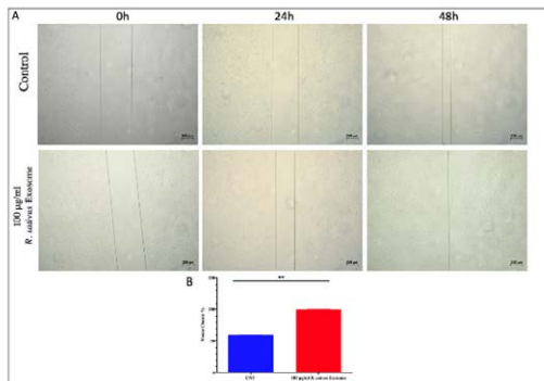
Figure 4. 5. (a) Images of scratch assay first 2 days under light microscope with 200 \mu\text{m} scale bar for control and 100 \mu\text{g}/\text{mL} radish exosome treated HC-OA cells. (b) Rate of closure HC-OA cells with radish exosome treated and untreated. Data are indicated with \pm SD, * P < 0.05 .
