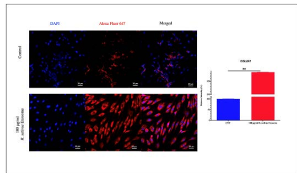
Figure 4. 12. ICC quantification and location of COL2A1 protein expression of HC-OA cells by confocal microscopy. All results were analyzed by two tailed multiple t tests. Data are shown with \pm SD, n=3
