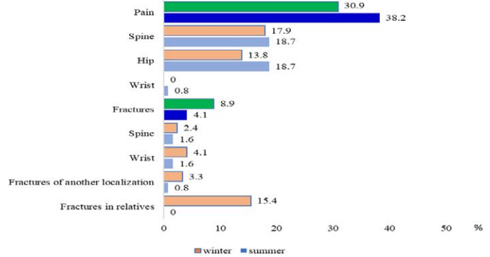
Figure. The frequency of pain and fractures of various localization depending on the season of the year.
