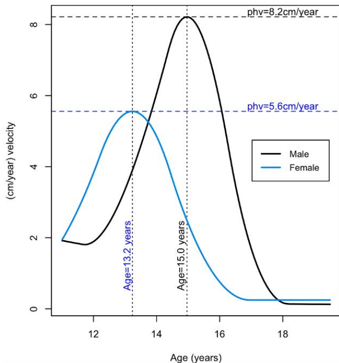
Figure 1. SITAR adjusted height velocity curves by sex
