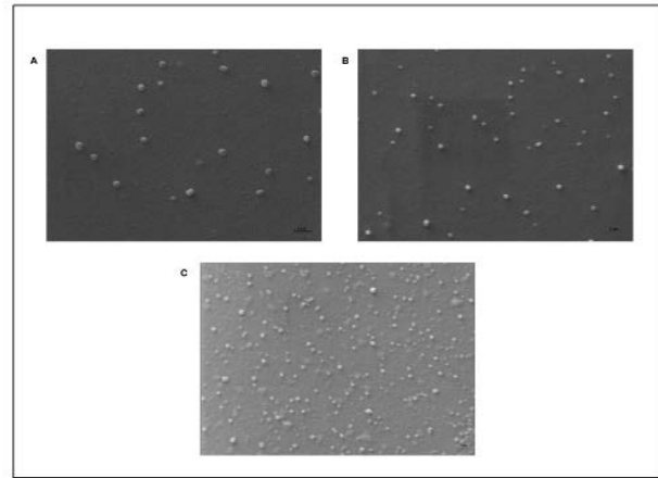
Figure 4.2. Morphology and sizes of (a) TELV, (b) LEVL, (c) RELV are indicated via Scanning Electron Microscope (SEM) with a scale bar of 1 \mu m.
