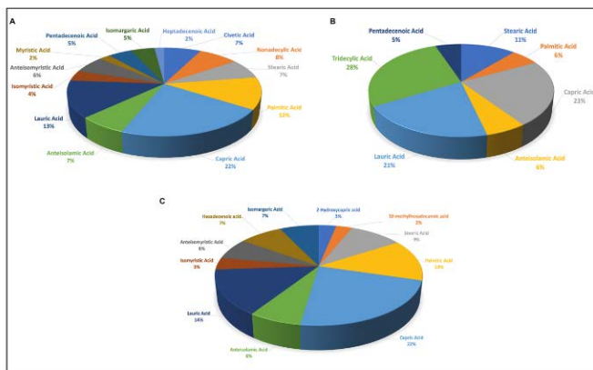
Figure 4.3. Fatty Acid Methyl Ester analysis for lipid contents of (A) TELV, (B) LELV and (C) REVL with percentages of leading lipid contents
