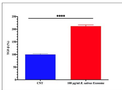
Figure 4. 9. TGF-β1 expression levels of HC-OA cells. Multiple t tests with two-tails were used to analyze the results. The data are shown with SEM, n=3, *P<0.05 and **P<0.01
