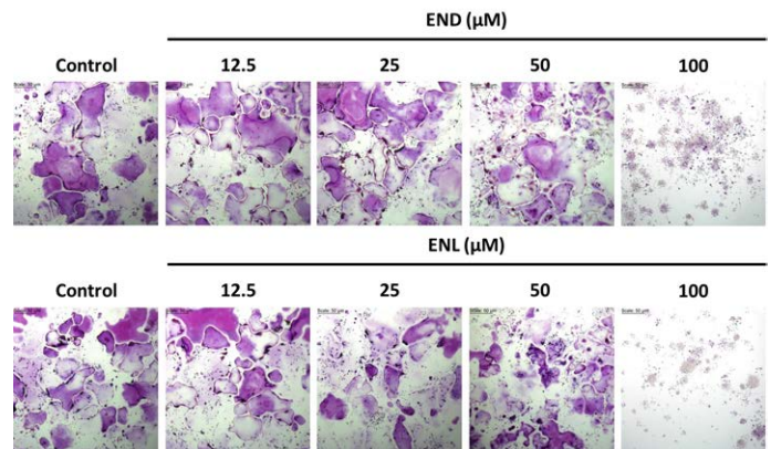
Figure 2. The inhibition effect of END and ENL on osteoclast differentiation.
