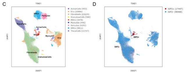
Figure 1. The analysis of integrated single-cell sequencing datasets from 13 different organs demonstrates that Igf2 exhibits high expression in mesenchymal stem cells. A. tSNE visualization analysis of the first-level clustering of single-cell transcriptomic sequencing results from 13 organs. B. Distribution of Igf2 across the 13 organs. C. UMAP visualization analysis of the second-level clustering of stromal cells. D. Specific high expression of Igf2 in the subpopulations of mesenchymal stem cells within stromal cells.
