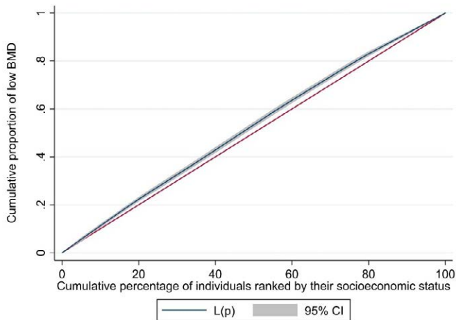
Figure 2. Lorenz curve illustrating SES inequality in low BMD
