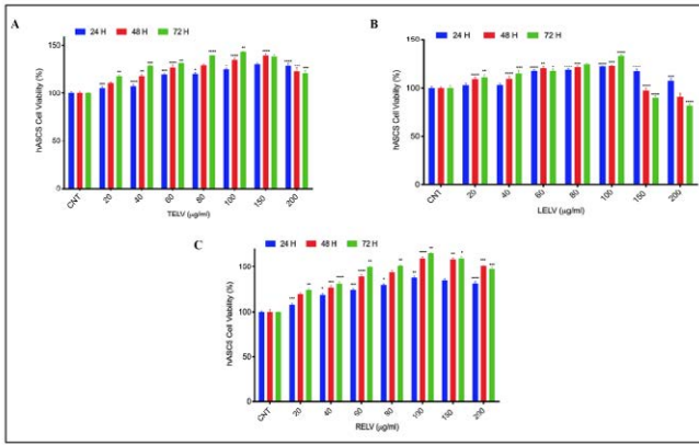
Figure 4.4. Effects of different doses between 20-200 µg/ml of (A) TELV (B) LELV (C) REVL on hASC proliferation after 24 h, 48 h, and 72 h incubation.
