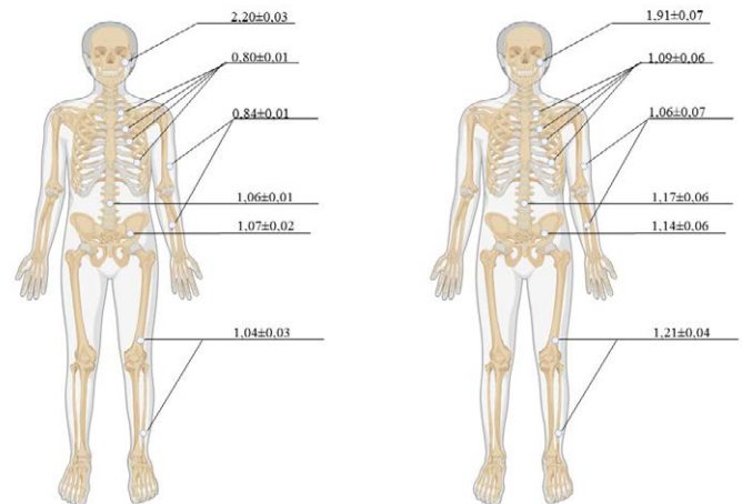
Figure 1. Distribution of aBMD values in men (right) and women (left) relative to body parts ( g/cm^2 )
