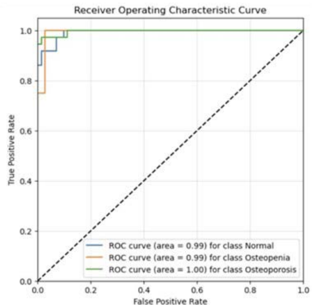
Figure 2. ROC curve for the model diagnosis accuracy. The AUCs
