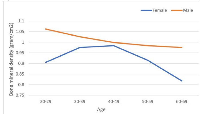
Figure 1. Comparison between males and females' neck of femur BMD at different age groups.
