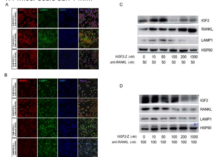
Figure 4. (A-B) CLSM images show the enrichment process of IGF2 and RANKL into lysosomes by 10nM anti-RANKL@iLYTAC. IGF2: red; RANKL: red; LAMP1: green. Scale bar=10μm (C) WB analysis of concentration-dependent human IGF2-Z (hIGF2-Z) and Anti-RANKL (fixed at 50 nM) on inducing RANKL and LAMP1 variation from cells in vitro . (D) WB analysis of concentration-dependent hIGF2-Z and anti-RANKL@iLYTAC (fixed at 100 nM) on inducing RANKL and LAMP1 variation from cells in vitro .
