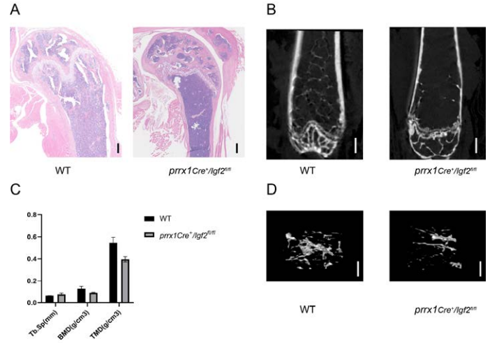
Figure 3. IGF2 deficiency promotes osteoporosis. (A) The representative of H&E staining in femora from Prrx1-Cre + Igf2 flox/flox mice and WT mice. Scale bars: 500 μm. (B-D) Representative μCT images (B,D) and quantitative μCT analysis of bone mass and microarchitecture (C) in femora from Prrx1-Cre + Igf2 flox/flox mice and WT mice. Scale bar: 1 mm.
