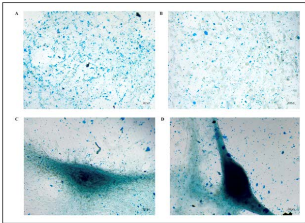
Figure 4. Alcian Blue staining images at 10X magnification of chondrogenic differentiations with (A) untreated cells, (B) treatment of LEVL, (C) treatment of TEVL, (D) treatment of RELV after 21 days.
