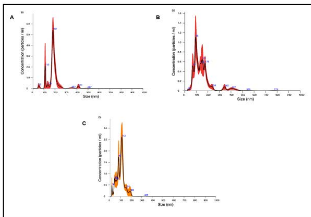
Figure 4.1. Size and concentration graphic data of (A) TELV, (B) LELV, (C) REVL are demonstrated via Nanoparticle Tracking Assay (NTA)
